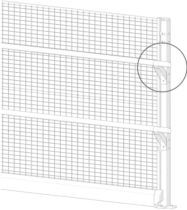
Handrail fittings with rivet, Page : 4
