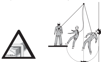
Figure 4: swinging risk
