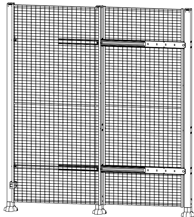
D46-XXX090
