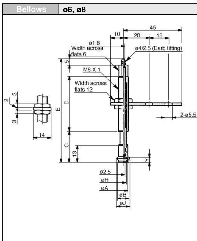
Bellows style
