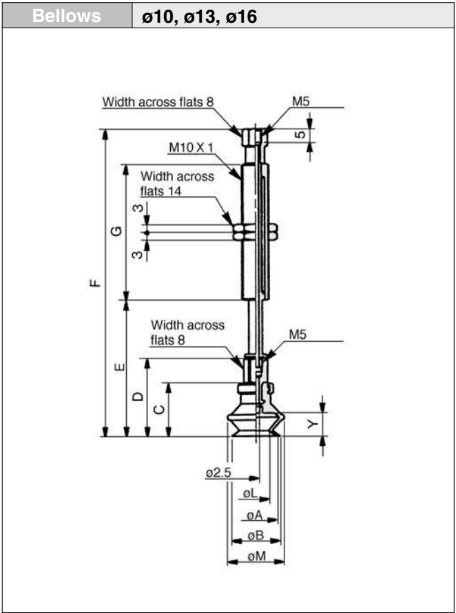
Bellows style
