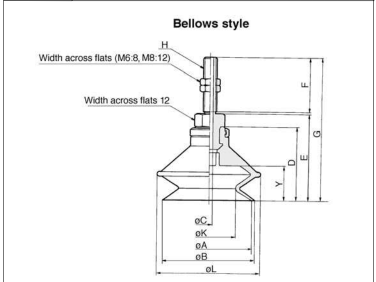
Pad Diameters ø40, ø50
