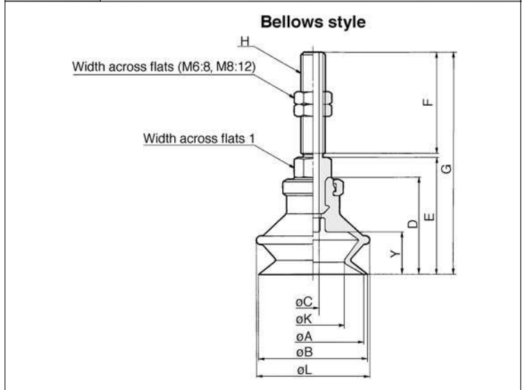
Pad Diameters ø20, ø25, ø32
