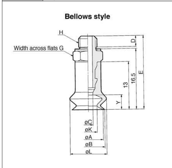
Pad Diameters ø6, ø8
