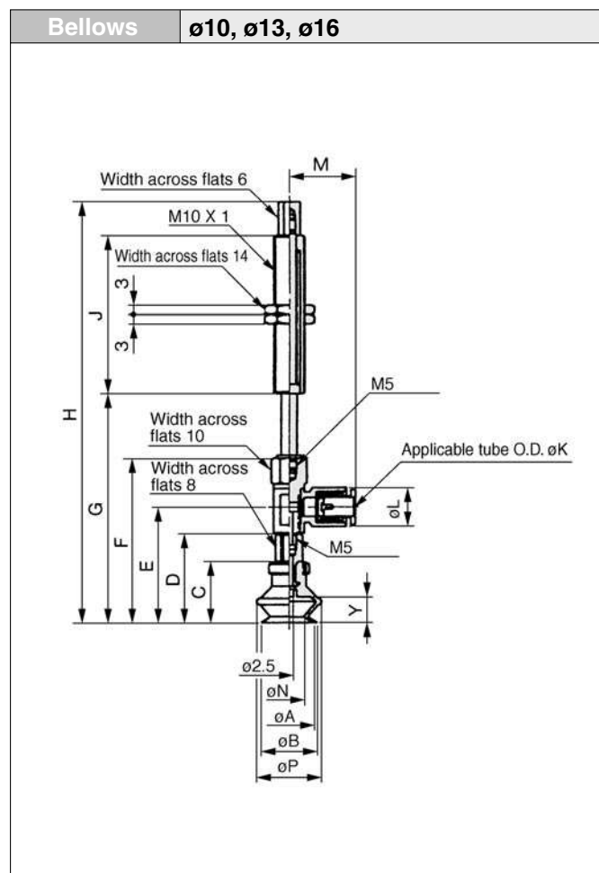
Bellows style
