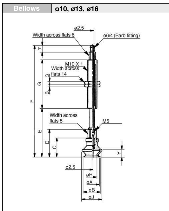
Bellows style
