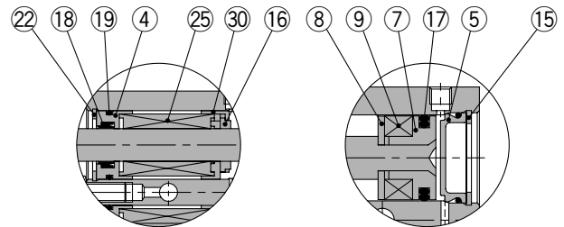
Rod cover
