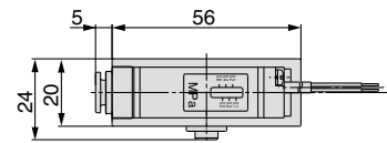
3-way valve common supply block + Pressure switch block (W)
