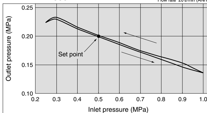
ARM11BA1-306-1 Conditions: Inlet pressure 0.5 MPa Outlet pressure 0.2 MPa Flow rate 20 \ell/\text{min} (ANR)
