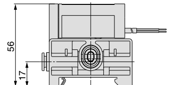
Common supply block with pressure switch (P)
