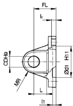
Mounting style (C)
