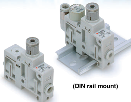
(Direct mount)
