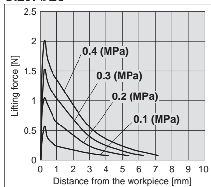
Size: \varnothing 25
