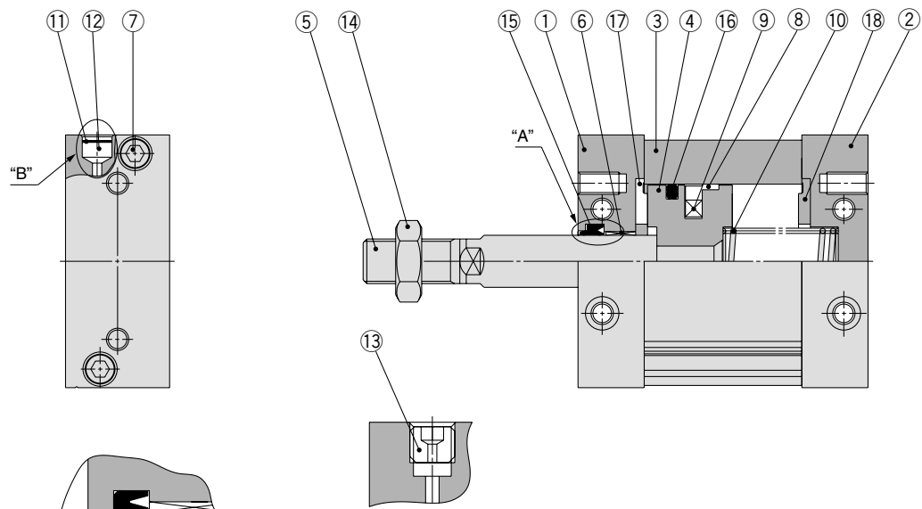
"A" section MU□25
