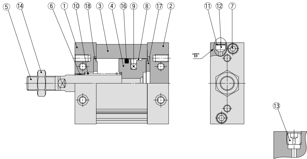
"B" section MU□25
