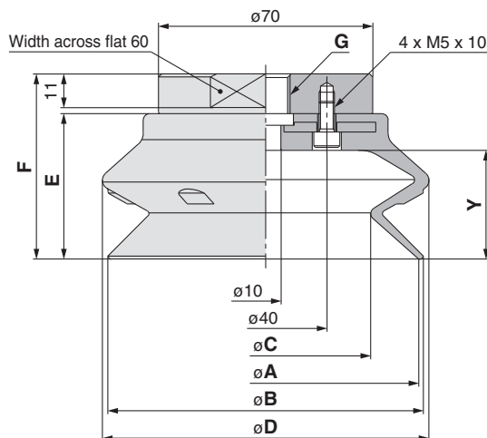
ZPT 100 125 HB□-B (Female thread)
