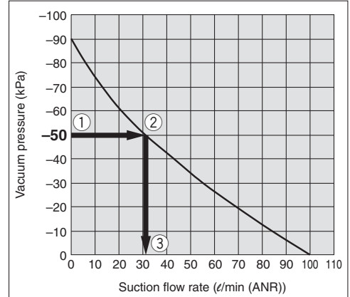
Chart 2. Selection Example by Min. Operating Flow Rate
