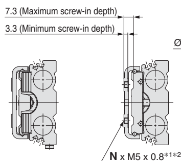
Cross-sectional view B-B
