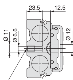
Cross-sectional view A-A
