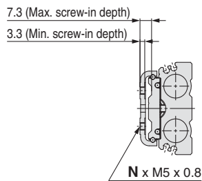
Cross-sectional view B-B
