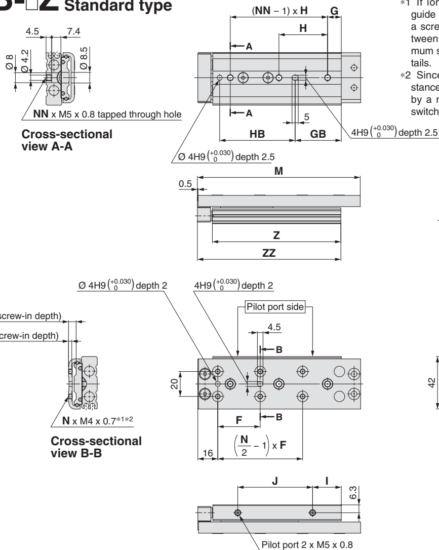
Bottom view of MXQ8B-40Z
