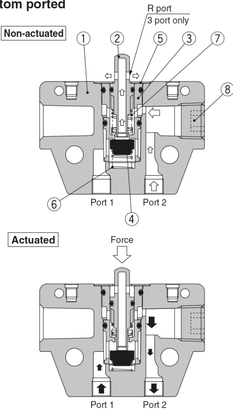
Bottom ported
