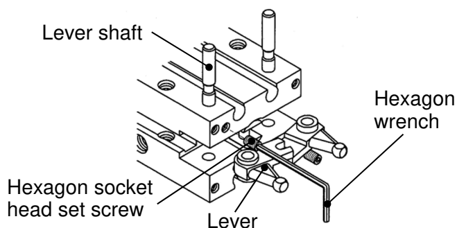
Hexagon wrench size
