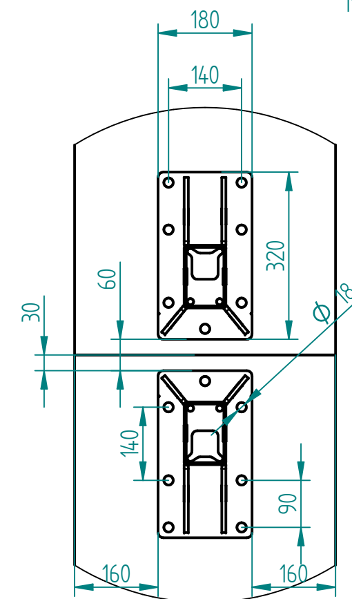
DETAIL C
