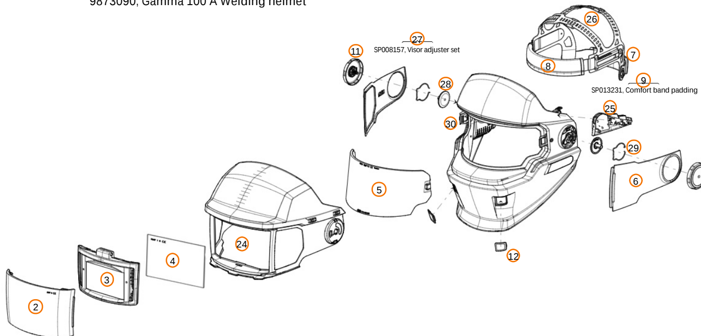
9873090, Gamma 100 A Welding helmet
